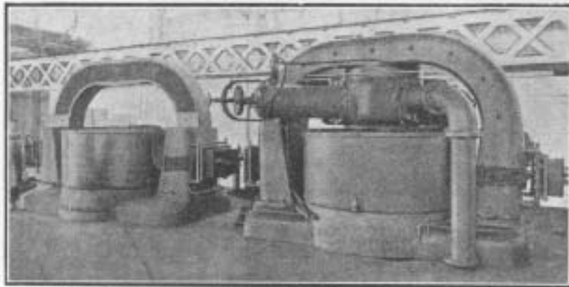
The Arc Converter of 500 Kilowatt 10 Capacity, at the Cavite Radio Station
